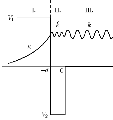
Figure 1. The regularized potential (3.1) and the eigenfunction (3.2).
