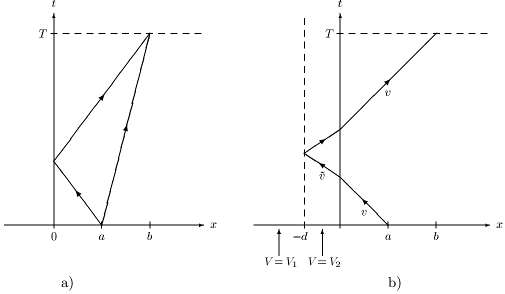
Figure 3. a) The direct and the bounce paths. b) The bounce path under the regularized potential (3.1).
