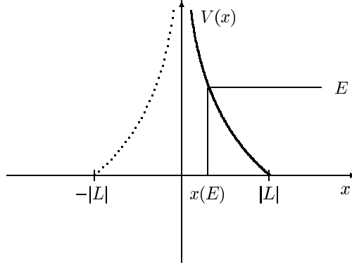
Figure 2. The realizing potential (4.7) is shown by the solid line for L > 0 . For L < 0 the obtained potential becomes the dotted line and is unphysical.
