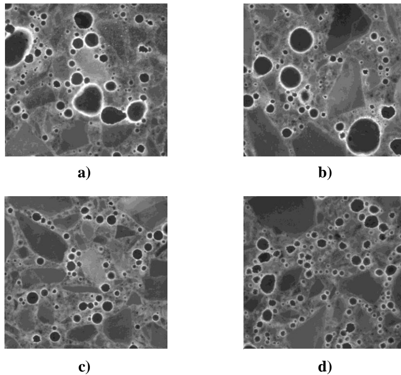
Fig. 4.9 Example photos of air bubbles in mortar specimens a) Simple method with SP1 and AE 0.006% (air 13.0%) b) Simple method with SP2 and AE 0.006% (air 12.0%) c) Water dividing method with SP1 and AE 0.01% (air 10.9%) d) Water dividing method with SP2 and AE 0.15% (air 13.4%)
