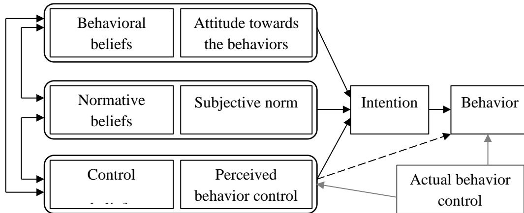
Fig. 7.1 conceptual model
