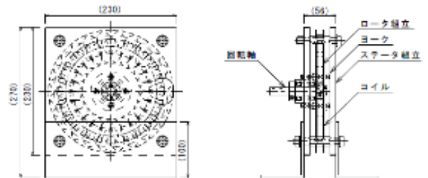
Fig.4.design drawing
